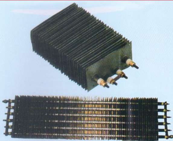
DUBLE U TYPE AIR FINDS HEATER TUBE 11mm / 8.2mm
